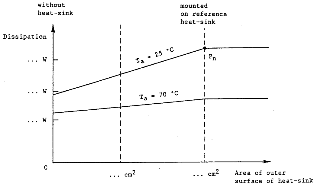
Figure 1: Heat-sink area derating curve
